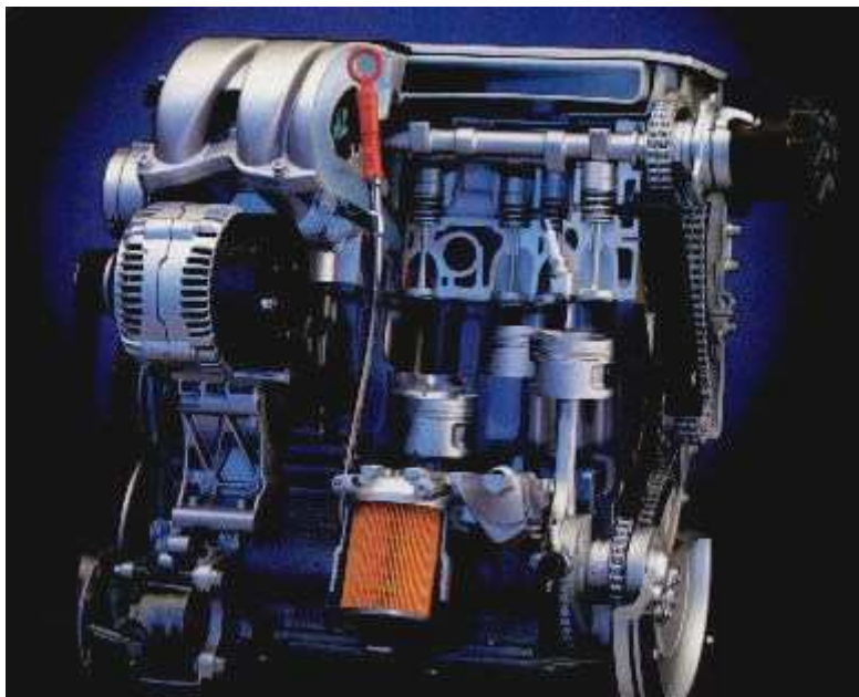
cutaway photo of an early generation 12v VR6
