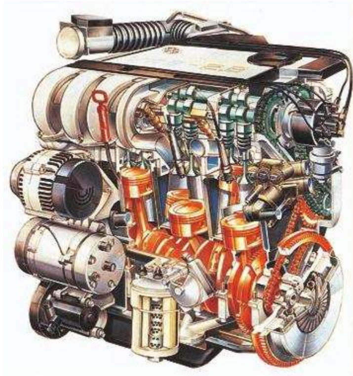
technical design diagram of the 12v VR6
