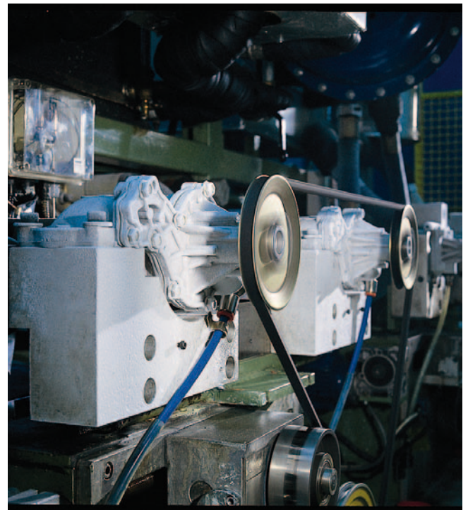
Test shock termico ( -40 C° / +140 C° ) Thermal shock test Choc test thermique Thermoschockversuche Test shock térmico
