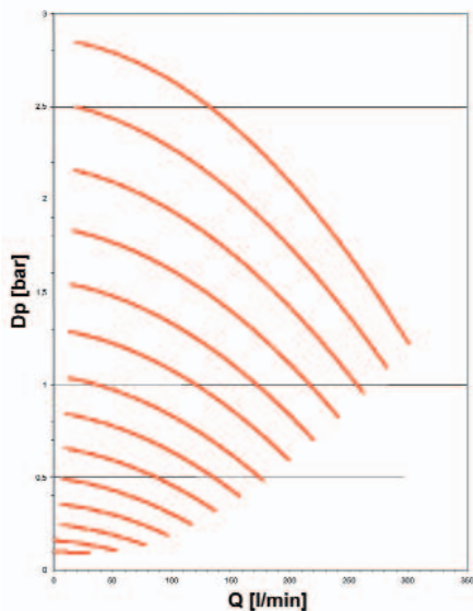
Curve Caratteristiche / Characteristic curves
