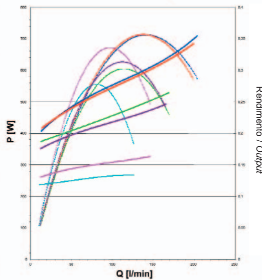
Curve Potenza n=5000 gir/min / Power curves n=5000 rpm
